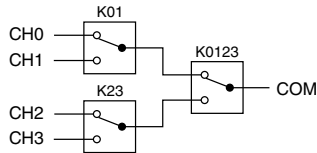
Figure 4. NI 2595 Power-On State
